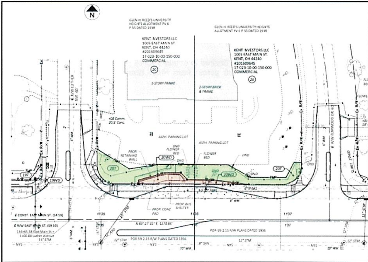
Figure 1 – Temporary (green) and permanent (pink) Right-of-Way from Starbucks Parcel
